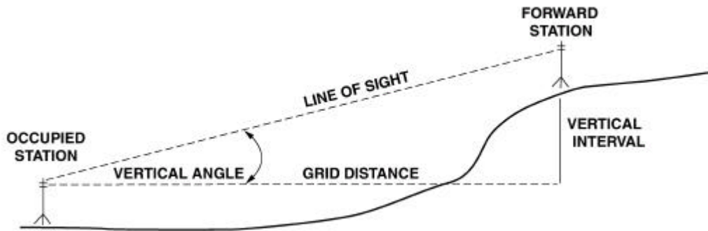
Figure 6-31. Elevation Triangle.
