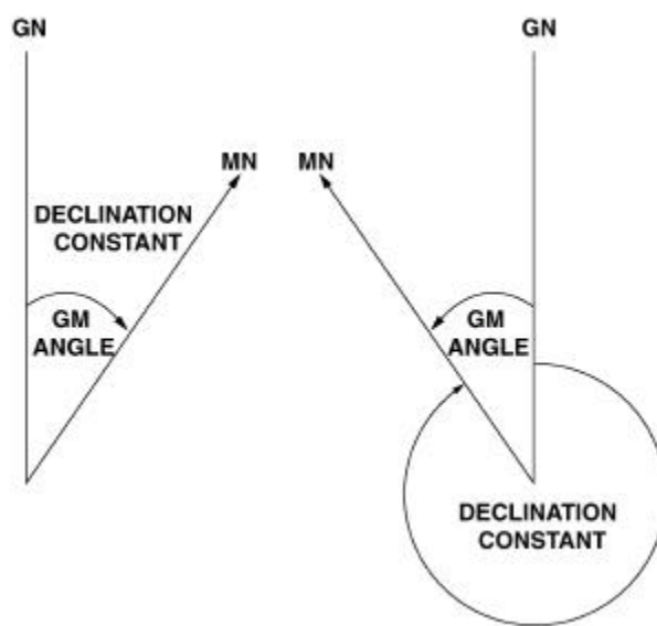
Figure 10-4. Relationship between a GM Angle and a Declination Constant.
