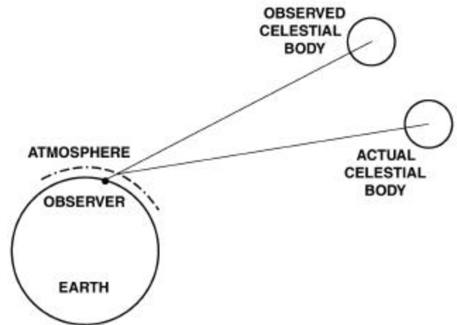
Figure 7-11. Refraction.
