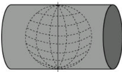
Figure 4-8. GK Projection.
