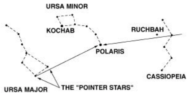
Figure 7-26. Identifying Polaris.
