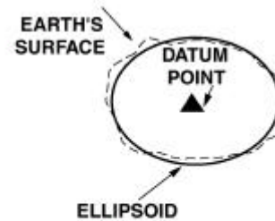
Figure 3-11. Geocentric Datum.
