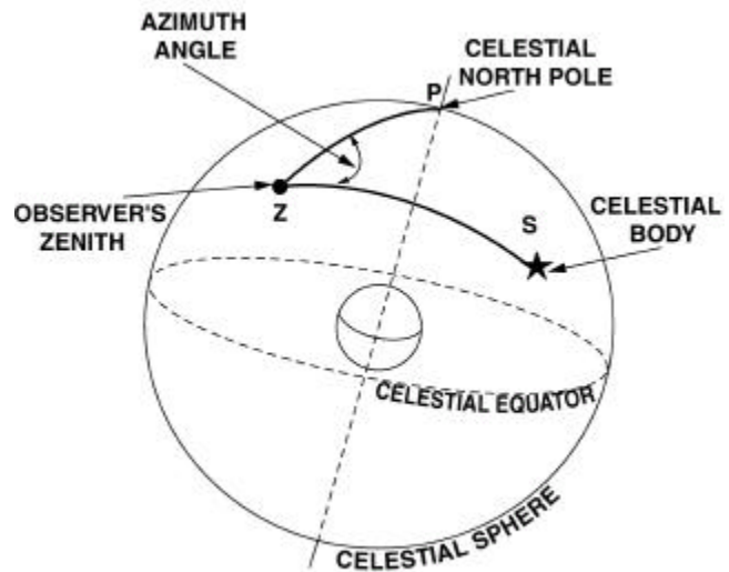
Figure 7-15. Azimuth Angle.
