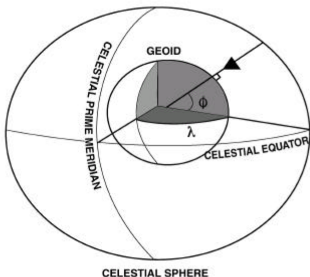
Figure 3-20. Astronomic Coordinates.
