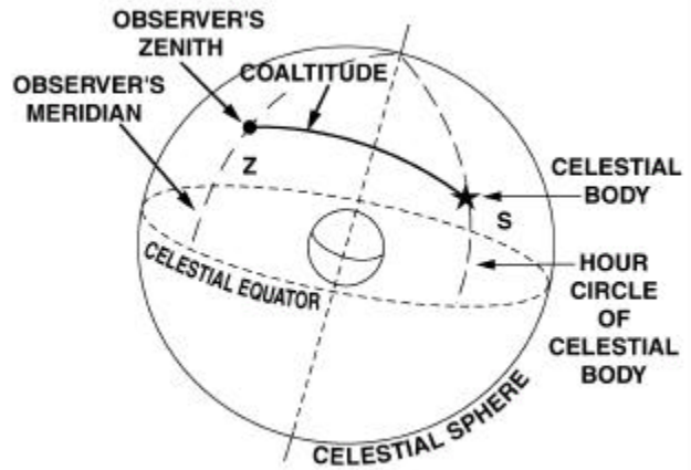
Figure 7-8. Coaltitude.
