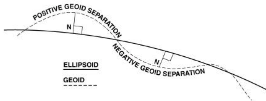
Figure 3-7. Geoid Separation.
