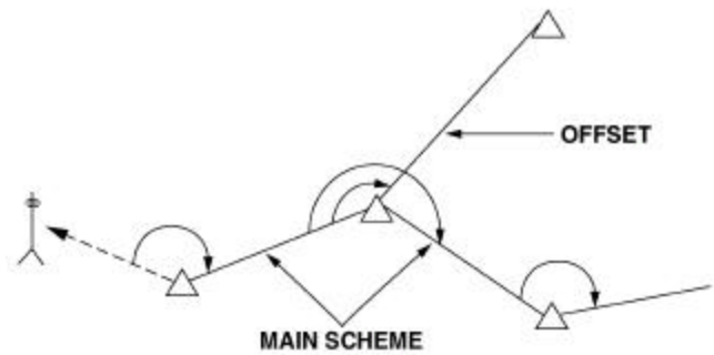
Figure 6-11. Traverse Legs.
