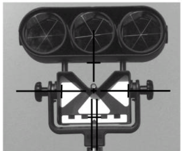
Figure 5-10. Pointings on a Target Reflector (GRZ3).
