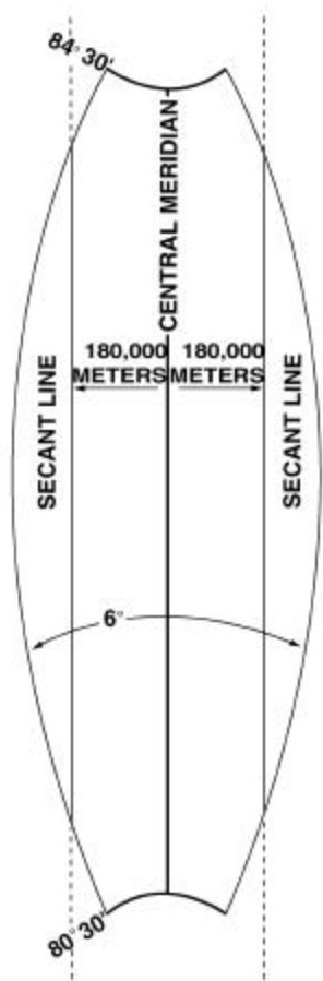
Figure 4-6. Secancy in a 6° Zone.
