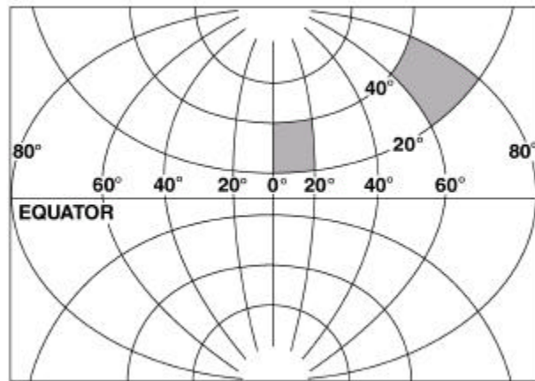
Figure 4-5. Distortion within the TM Projection.
