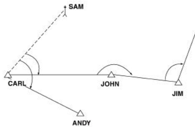
Figure 6-36. Offset Legs.
