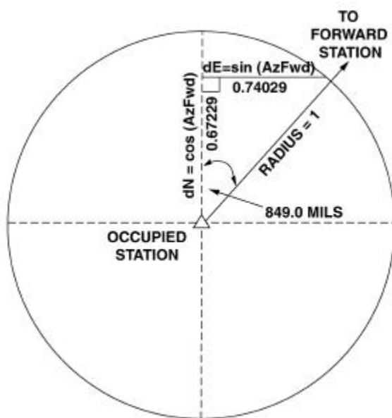
Figure 6-32. Value of Trigonometric Functions of Angles.
