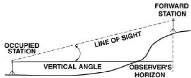
Figure 6-7. Vertical Angles.
