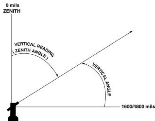
Figure 5-14. Vertical Readings/Angles.
