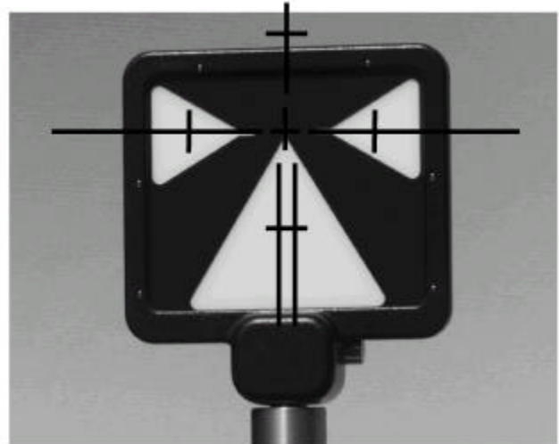
Figure 5-9. Pointings on a Target Plate (GZT1).
