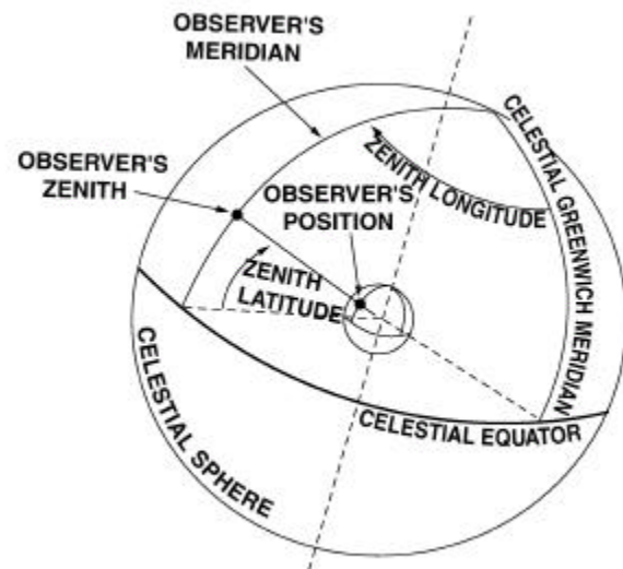
Figure 7-3. Zenith Position.
