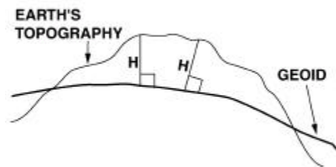
Figure 3-2. Elevation.
