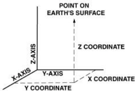
Figure 3-14. Cartesian Coordinates.
