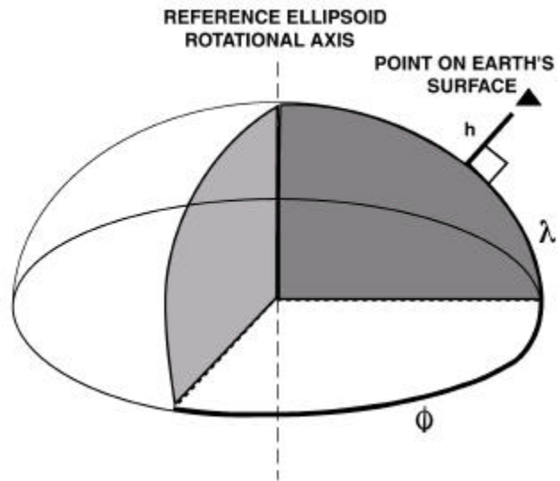
Figure 3-15. Geographic Coordinates.
