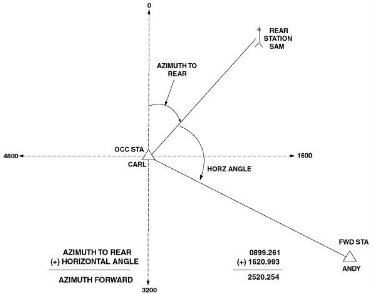
Figure 6-29. Azimuth-Angle Relationship.
