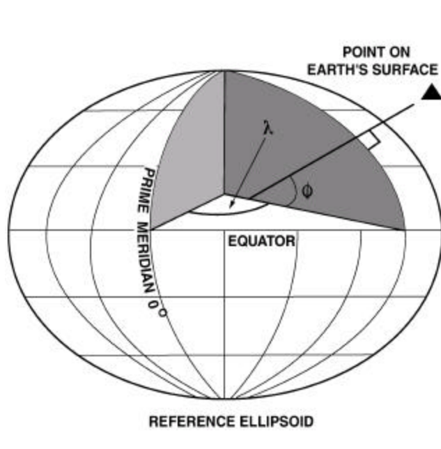
Figure 3-19. Geodetic Coordinates.
