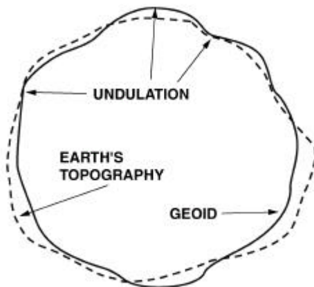
Figure 3-1. Undulation.
