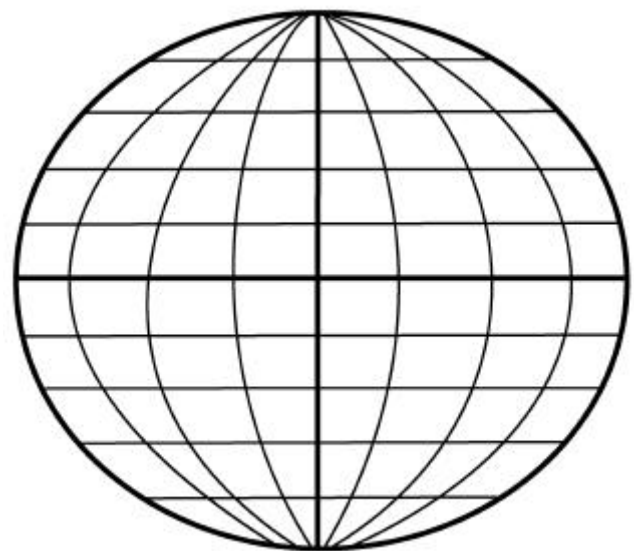
Figure 3-18. Graticule.
