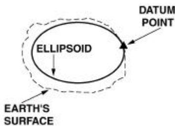
Figure 3-10. Surface-Fixed Datum.
