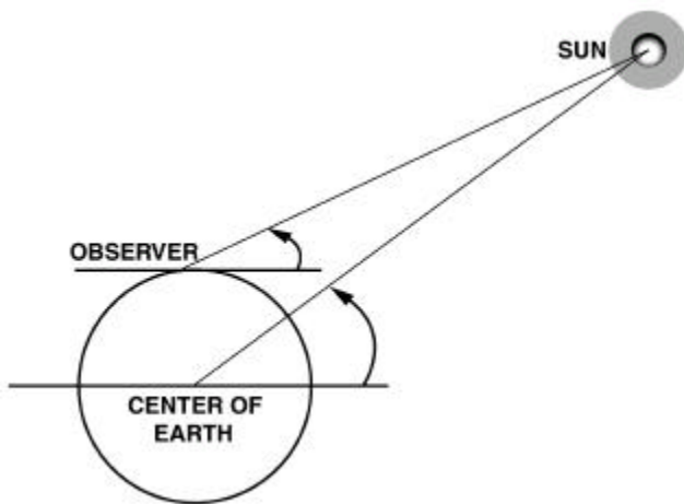
Figure 7-10. Parallax.
