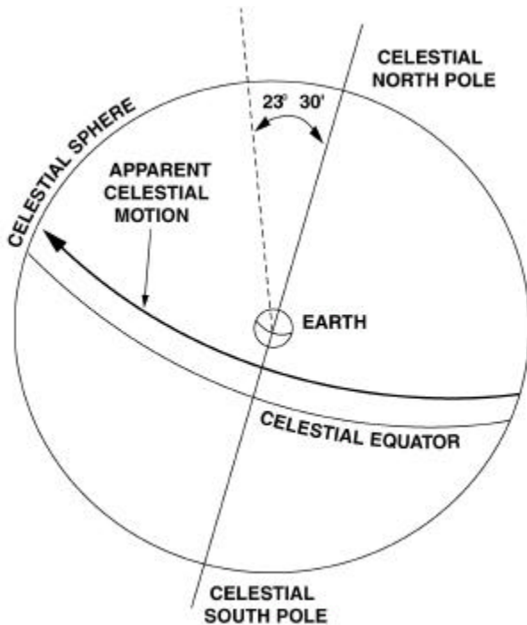
Figure 7-2. Celestial Sphere.
