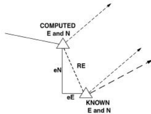
Figure 6-39. Pythagorean Theorem.
