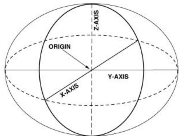
Figure 3-13. Coordinate Planes.
