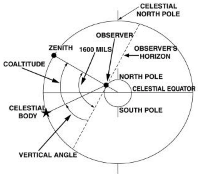
Figure 7-9. Determining Coaltitude.
