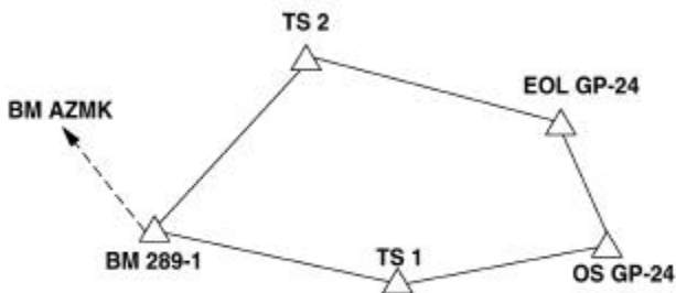
Figure 6-4. Closed Traverse on the Starting Point.
