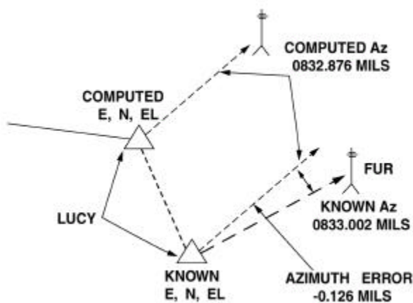
Figure 6-41. Azimuth Error.
